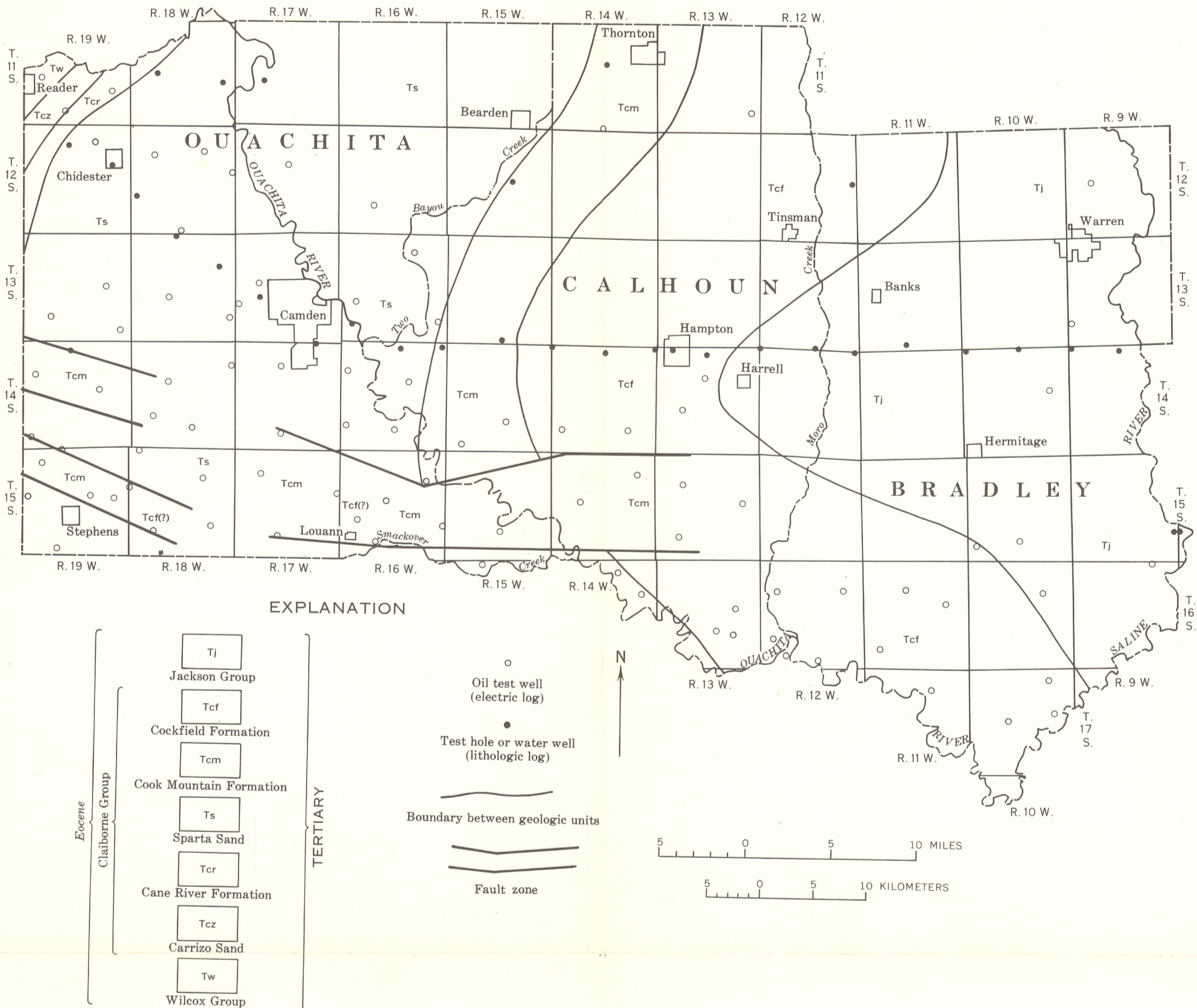
MAP SHOWING DISTRIBUTION OF GEOLOGIC UNITS AT THE LAND SURFACE OR DIRECTLY BENEATH THE QUATERNARY SYSTEM IN BRADLEY, CALHOUN, AND OUACHITA COUNTIES, ARKANSAS
